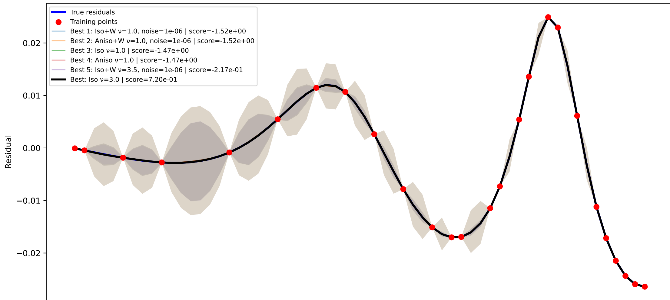
GPR kernel comparison node=4 RMSE=1.450e-05, train RMSE=1.803e-11
